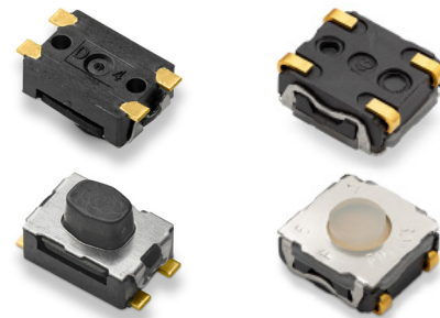
Figure 1: Gold Plated KMR723NG LFG and KSC253G SP DELTA LFG Tactile Switches
